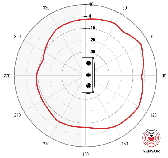
Elevation - 5 GHz
