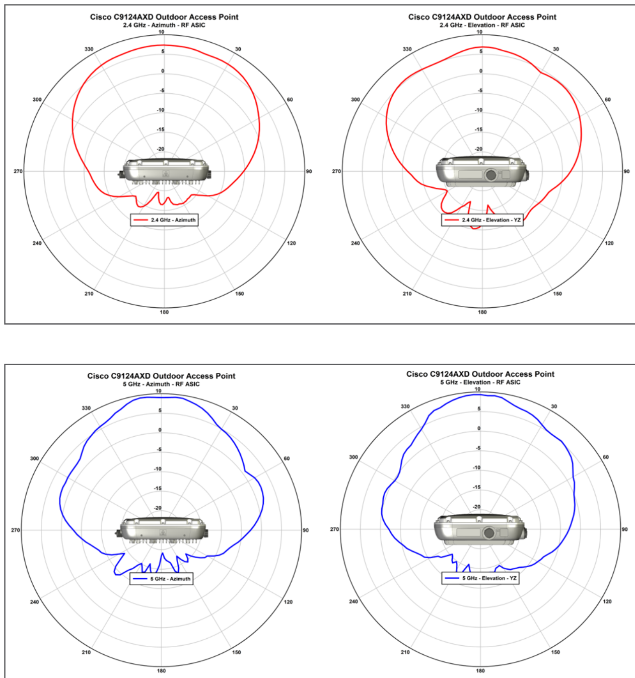
Figure 2. Antenna profiles
