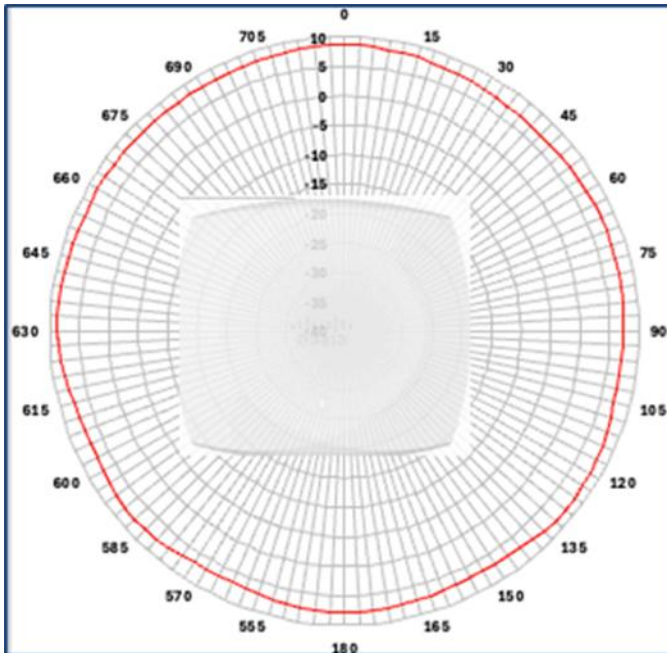
Figure 1. Antenna patterns
