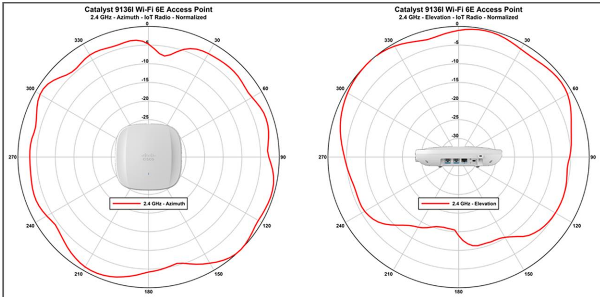
Figure 2. Antenna profiles
