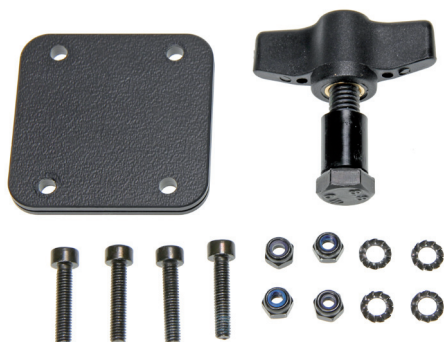
Item no 215676 Wingnut and distance plate for mounting on Suction Cup Mounts (item no's 215671 & 215675). Nuts, bolts, and lock washers included.
