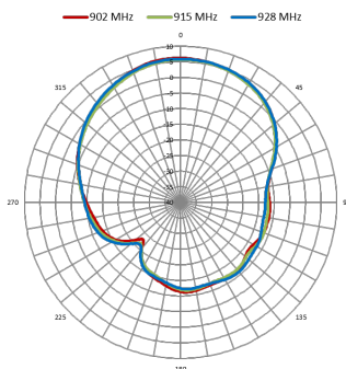
Horizontal (LHCP)
