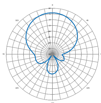
Horizontal (FCC)
