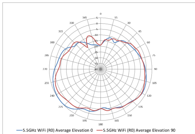
5.5GHz Wi-Fi antenna patterns (vertical)
