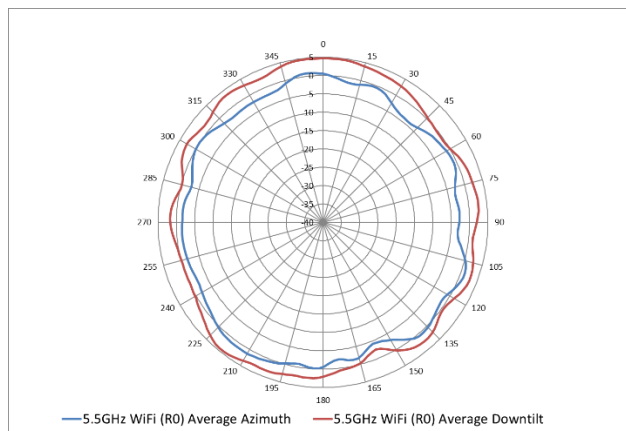
5.5GHz Wi-Fi antenna patterns (horizontal)
